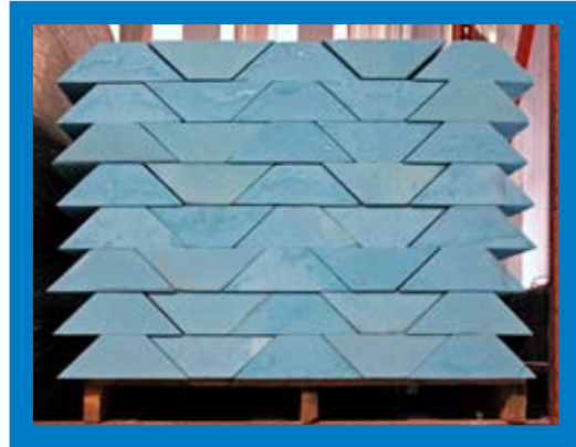
Pre-cut foam was integrated into the circumference of each section to help form exterior structural ribs that help support the liner.
